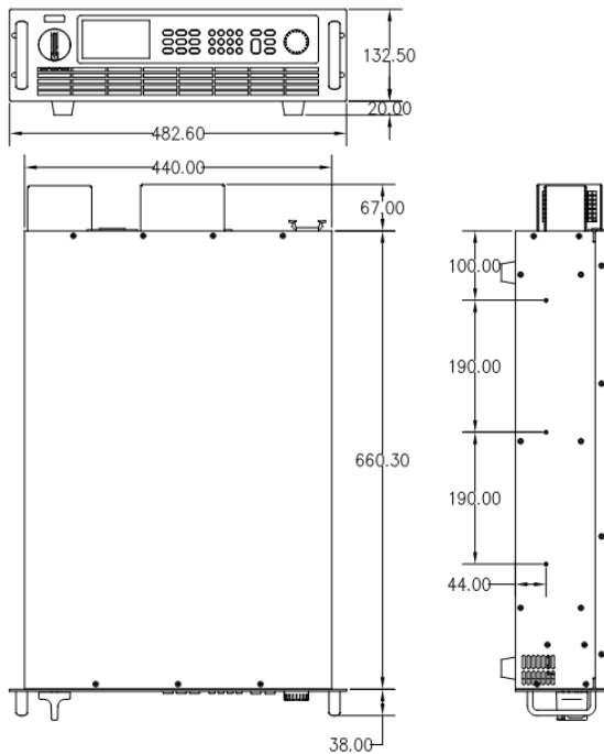
Dimensions for 5kW~18kW model
