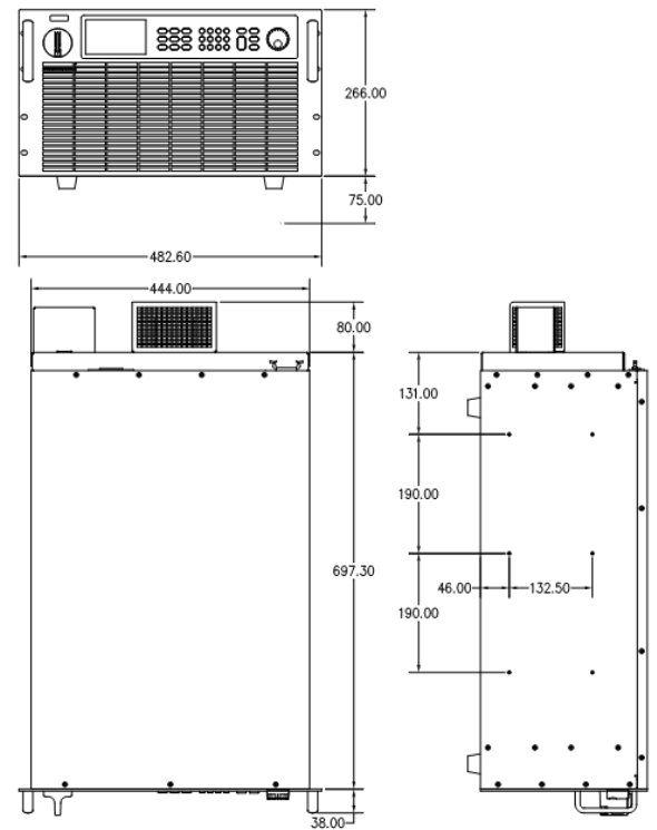
Dimensions for 20kW~36kW model
